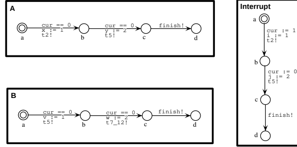
Fig. 7. Dealing with interrupts
