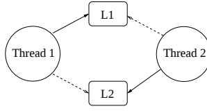
Fig. 4. Classical deadlock where task 1 takes lock L1 first and task 2 takes lock L2 first.
