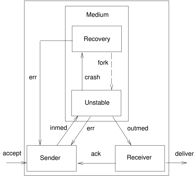
Figure 2: The Protocol
