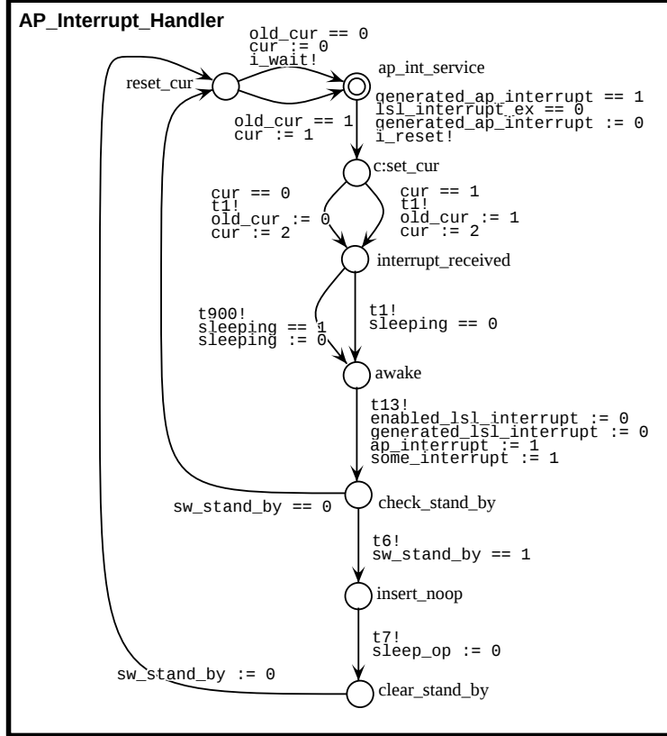
Figure 5.5: The AP Interrupt Handler
