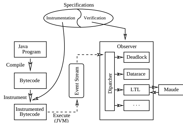
Figure 1: JPAX Architecture
