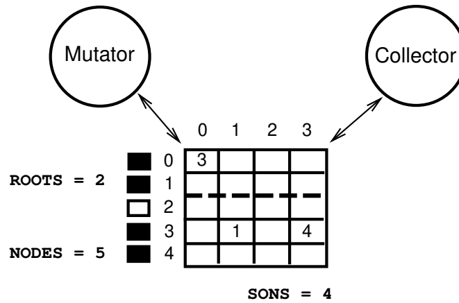
Figure 2.1: The Mutator, Collector and Shared Memory
