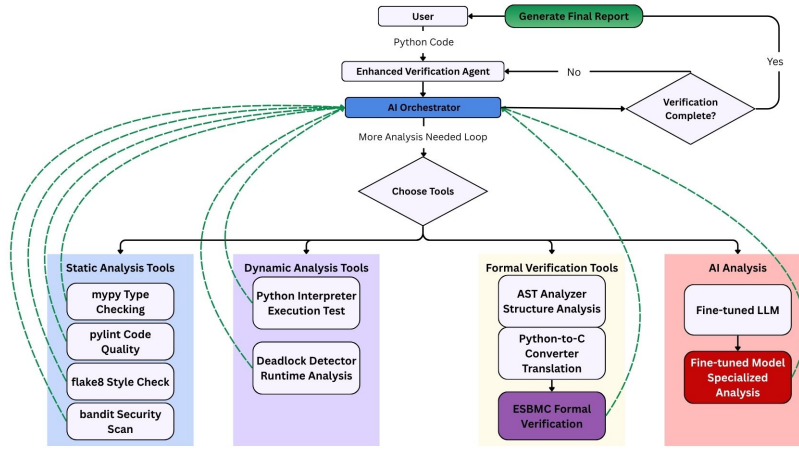
Fig. 2. Complete System Architecture. The LLM orchestrator coordinates verification by routing analysis through four tool categories based on code characteristics: Static Analysis, Dynamic Analysis, Formal Verification, and AI Analysis. The system iterates up to 10 times, synthesizing results until verification objectives are met, then generates a final report.
